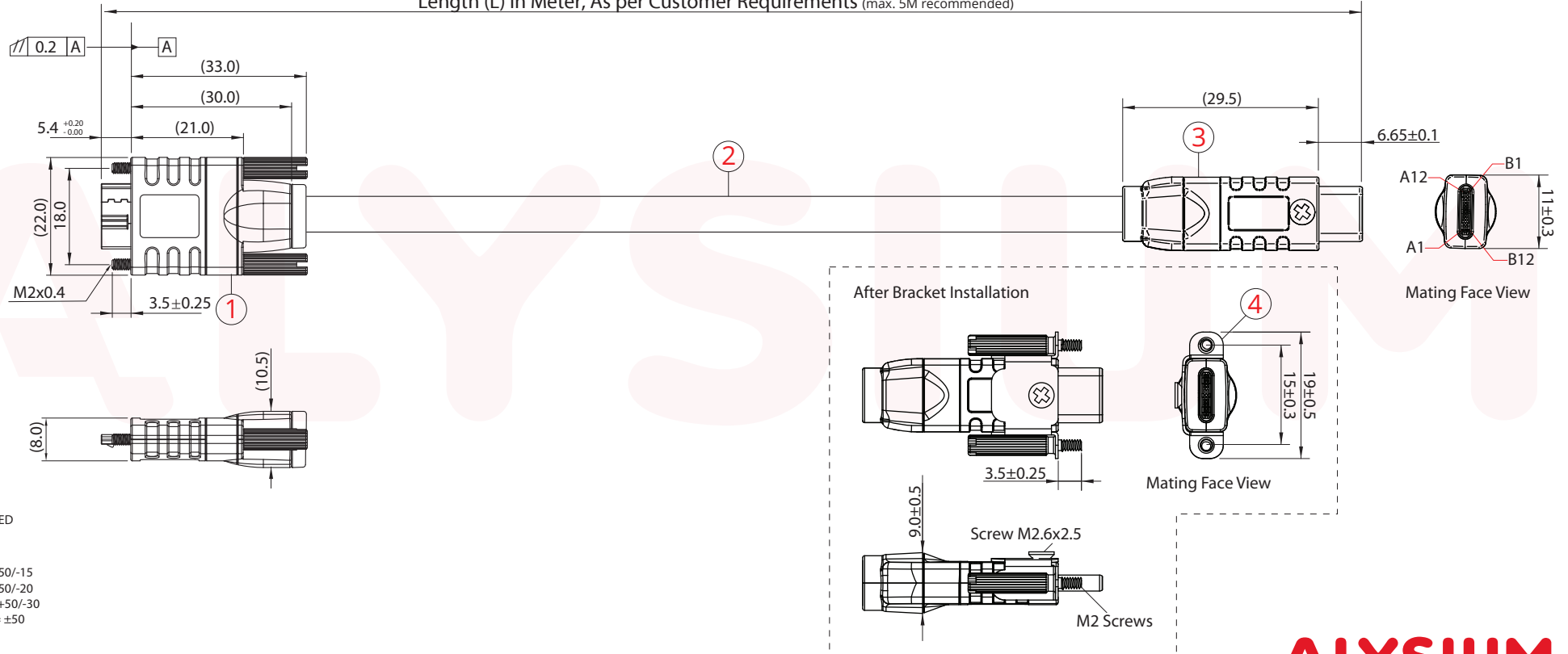
Mating Face View
