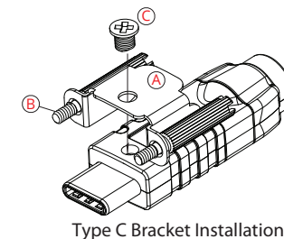
Type C Bracket Installation
